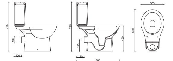
TR03KLZ00 | TR04KLZ00 TRIA RIMLESS DUVARA YARIM DAYALI KLOZET | TRIA RIMLESS SEMI BACK TO WALL CLOSET TRO2RZV00 | TRO2RZV00 REZERVUAR | CISTERN
