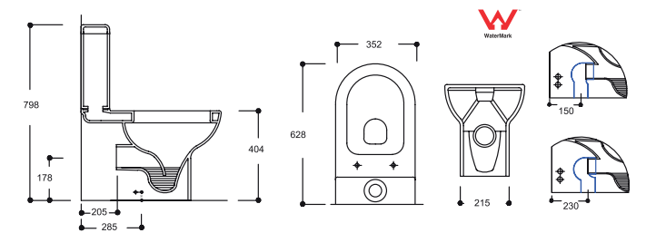
K005KLZ00 COMPACT DUVARA DAYALI KLOZET
