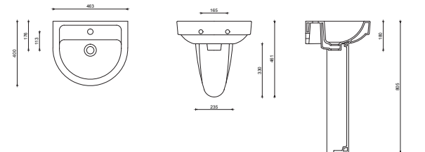
TP09LVB01 COMPACT BANTLI LAVABO (40x46) K001AYK00 KOLON AYAK K002AYK00 YARIM AYAK TP09LVB01 COMPACT WASHBASIN "D-SHAPED" (40x46) K001AYK00 PEDESTAL K002AYK00 SEMI PEDESTAL
