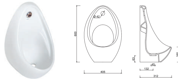
TP05PSR00 | TP05PSR00 ANKASTRE FOTOŞELLİ PİSUVAR | BUILT - IN SYPONIC URINAL
