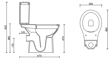
CA19KLZ00 | CA20KLZ00 CARMINA RIMLESS ENGELLİ KLOZET (ARKA ÇIKIŞLI) | CARMINA RIMLESS DISABLED CLOSET (P-TRAP) CA09RZV00 | CA20RZV00 REZERVUAR | CISTERN
