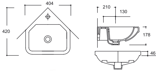
TP03PLV01 PUZZLE LAVABO (30x43) SOL TP03PLV01 PUZZLE BASIN (30x43) LEFT
