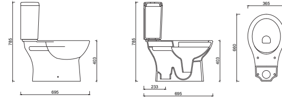
TR23KLZ00 | TR24KLZ00 TRIA RIMLESS DUVARA DAYALI KLOZET | TRIA RIMLESS UNIVERSAL REZERVUAR | BACK TO WALL CLOSET TRO2RZV00 | TRO2RZV00 KLOZET + REZERVUAR | CISTERN
